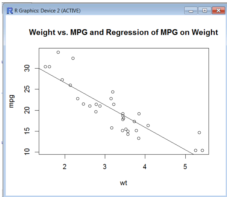
Display 8. R ATTACH and PLOT command output with regression and title added
