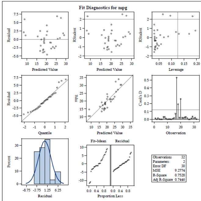
Display 10. SAS PROC REG analysis output
